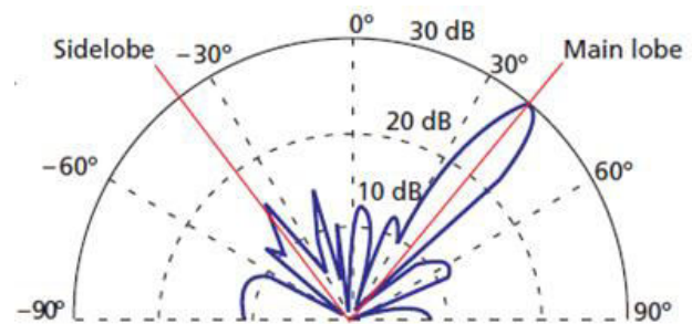
Fig. 3. Typical directional sensitivity profile with the main focused direction.
