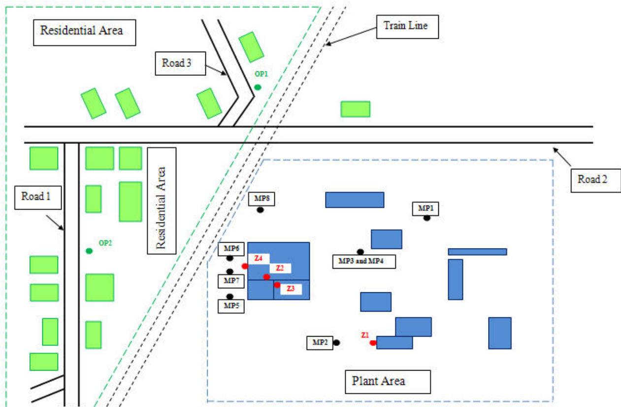
Fig. 9. Site map with measurement points and position of main noise sources.
