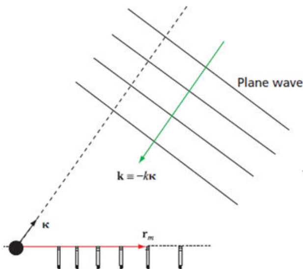
Fig. 2. The grid microphones, focused on the far field and flat wave coming from the focused direction.
