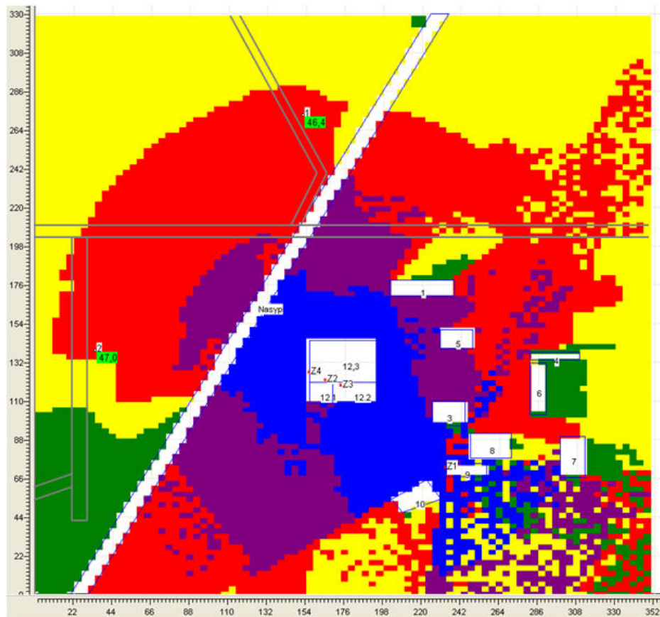
Figure 10. Acoustic map without noise sources reduction measures.
