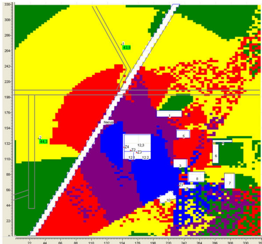
Fig.11. Acoustic map with assumed noise reduction for sources Z2, Z3 and Z4.
